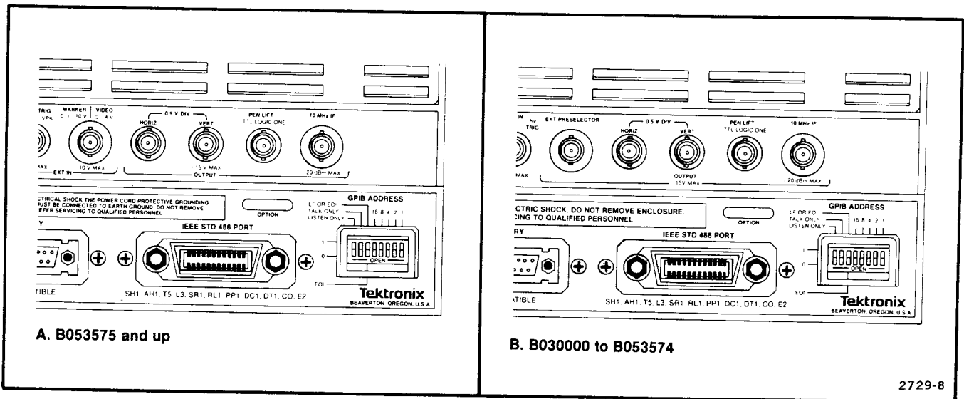
Fig. 3-18. The 492P GPIB Port and Switches.
