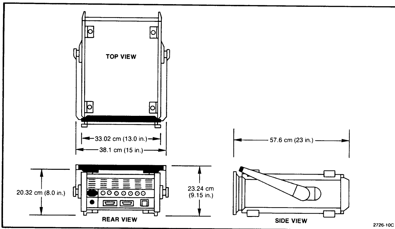
Fig. 1-2. Dimensions.
